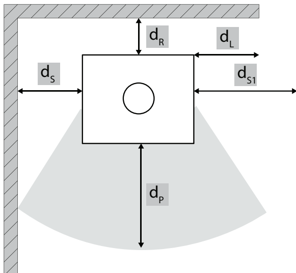
ODYN, ODYN L - DISTANCES TO COMBUSTIBLES; position layout 1
