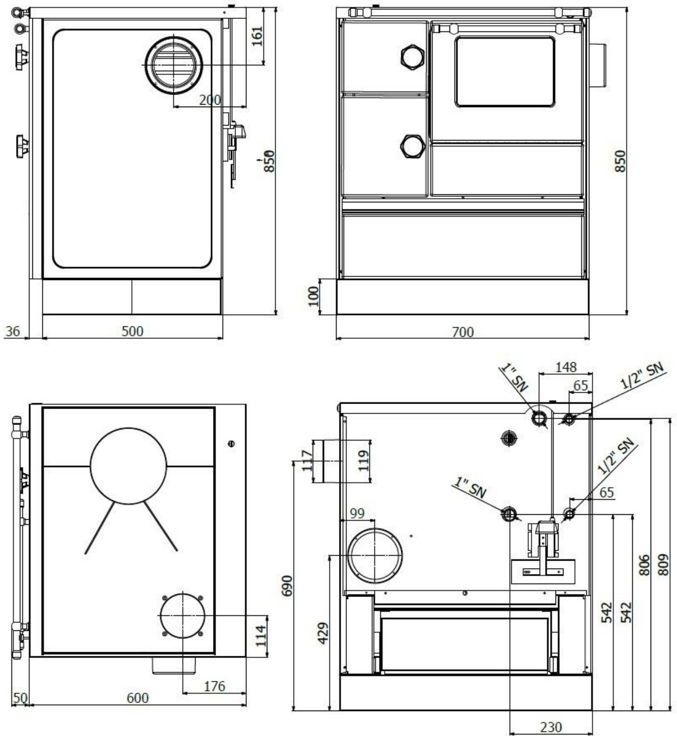
Figure 1 - Dimensions
